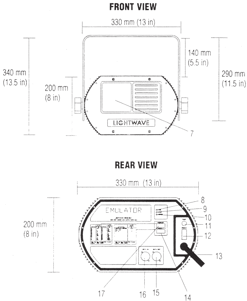
Emulator Fixture Illustration: Front View & Rear View (See Appendix A for fixture specifications.)
